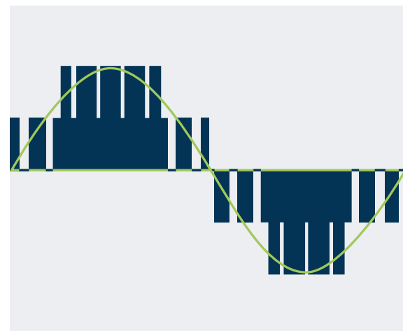
Waveform output voltage
