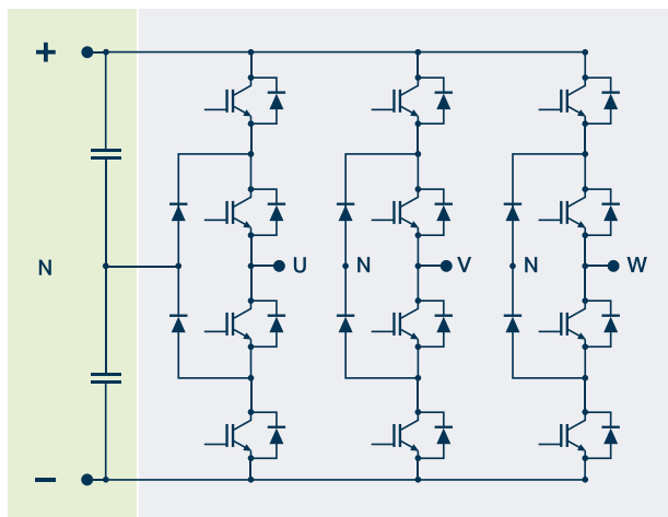
Circuit 3 – Level inverter
